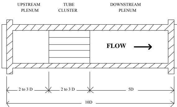
Figure 2 Typical Flow Straightener
